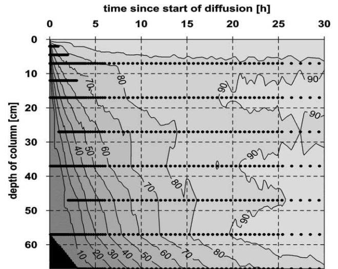
Fig. 3. Diffusion of ambient oxygen into a soil column where ground air has been replaced by nitrogen prior to experiment. Contours show oxygen saturation (100% is equivalent to p_{O_2} = 0.21 ). Filled circles show measurements. Seven optodes were used simultaneously. Switching between sensors was conducted with array described above (LAFOSS).
