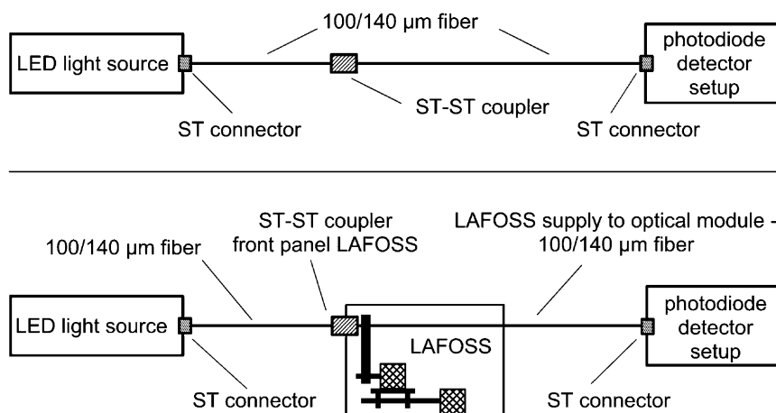
Fig. 2. Experimental setup for attenuation measurements. Top: setup for reference measurement without LAFOSS; bottom: setup with LAFOSS.
