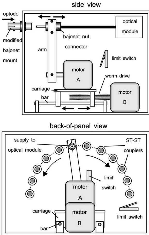
Fig. 1. General structure of the very low attenuation fiber-optical sensor switch (LAFOSS). Above: side view; below: back-of-panel view.
