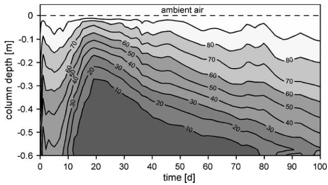
Fig. 7. Pyrite weathering in soil column experiment — development of oxygen concentrations (% air saturation) over time and depth. Measurements with calibrated micro-optodes.
