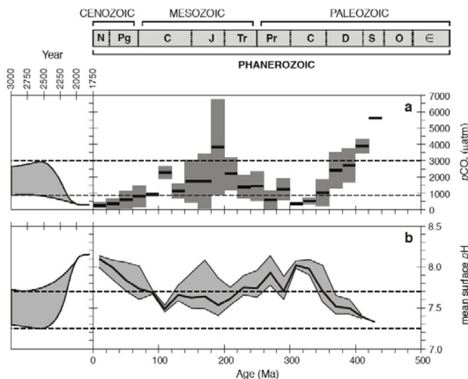
Fig. 4. Geologic history and projection of (a) atmospheric p\text{CO}_2 and (b) modeled changes in pH over the same time period. Horizontal dashed lines indicate the range of predicted p\text{CO}_2 peak atmospheric \text{CO}_2 concentration over the next century. Dark lines are average historical p\text{CO}_2 values, while gray shading indicates \pm one standard deviation. After Ridgwell and Zeebe (2005).
