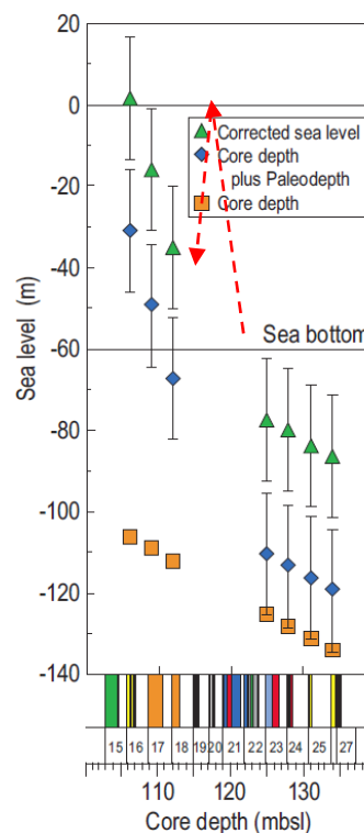
Fig. 3. Sea-level changes during Termination II (TII), reconstructed using a new shallow-water sequence found from offshore Tahiti by IODP Exp. 310 (Fujita et al., submitted; Iryu et al., submitted). Dotted red lines indicate a sea-level reversal event midway through TII.
