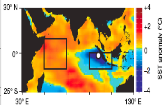
Fig. 2. Indian Ocean Dipole (IOD)
