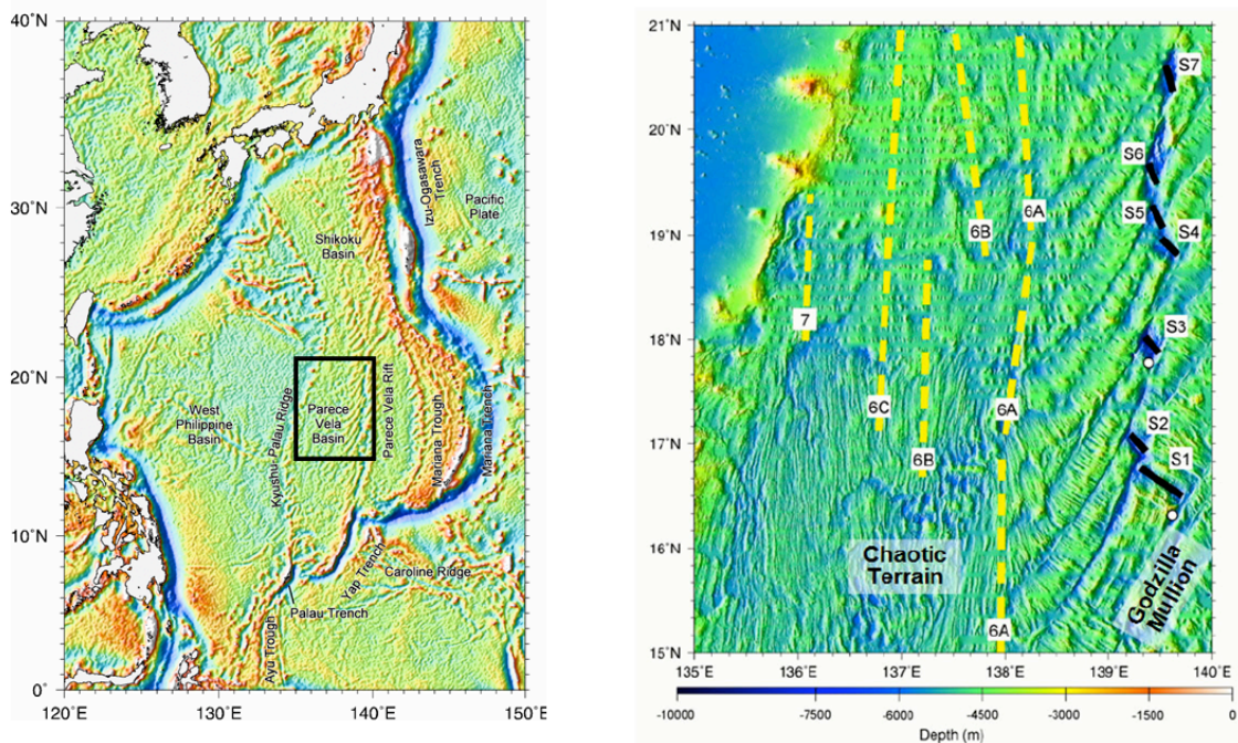
Fig. 1. Index map of the Philippine Sea and the bathymetry of the Parece Vela Basin. Yellow dashed lines in the right panel are magnetic anomaly isochrons. The first order segments of the Parece Vela Rift are labeled S1 to S7 by Ohara et al. (2001). Godzilla Mullion occurs on S1.
