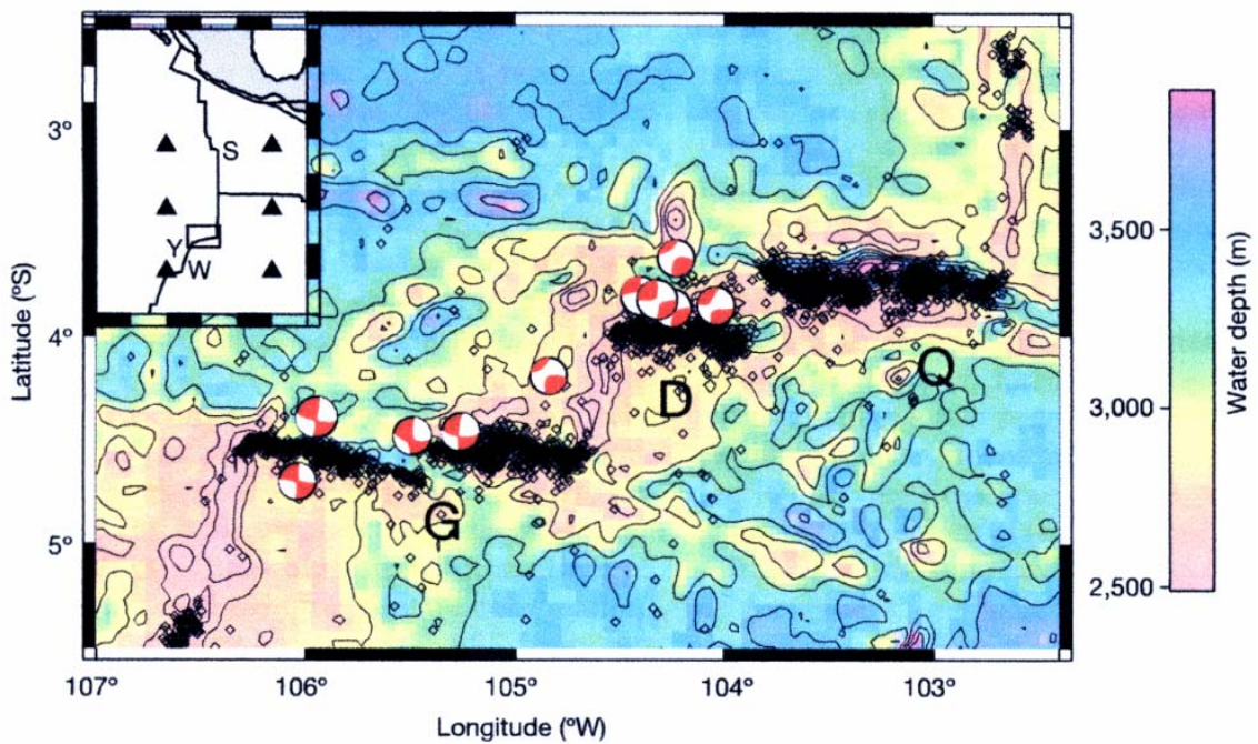
Figure 2. Seismicity near the on transform faults of the East Pacific Rise. (McGuire et al., 2005).
