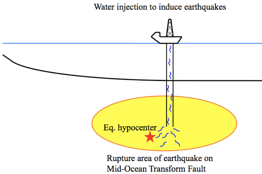
Figure 1. Schematic of water injection experiment to induce earthquakes.
