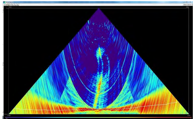
Figure 4: As shown in previous research, the Håkon Mosby Mud Volcano is a fairly active volcano. It is known for gas emissions, which we could clearly see in the triangular multi-beam swath by several curved "flares" in the center.
